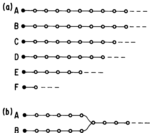
Figure 1: a. One-to-one computation. The left-hand end of a horizontal chain represents the initial state, and forward computation represents motion to the right, through a sequence of states represented by successive open circles. Different capital letters correspond to different initial states, that is, different programs. b. Information-discarding junction. Two computational paths, moving to the right, merge into one.
